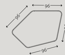
FREEo05 island left 170x125xHs 38 cm
